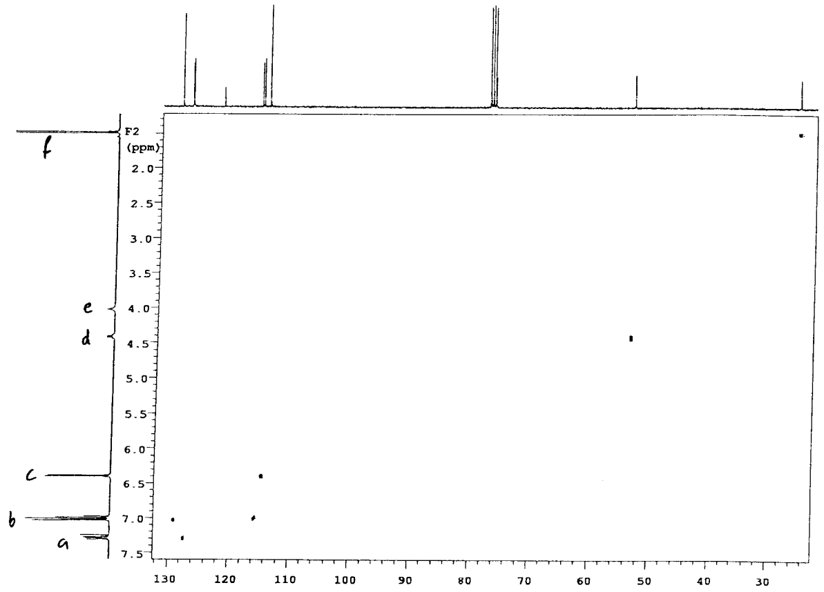
HSQC
