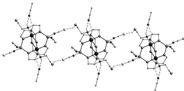
Figure 3. Fragment of the hydrogen-bonded chain in 2 .
