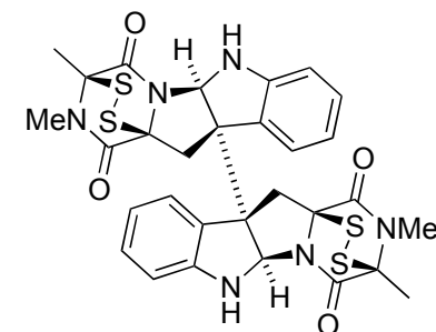
(+)-11,11'-Dideoxyverticillin A
