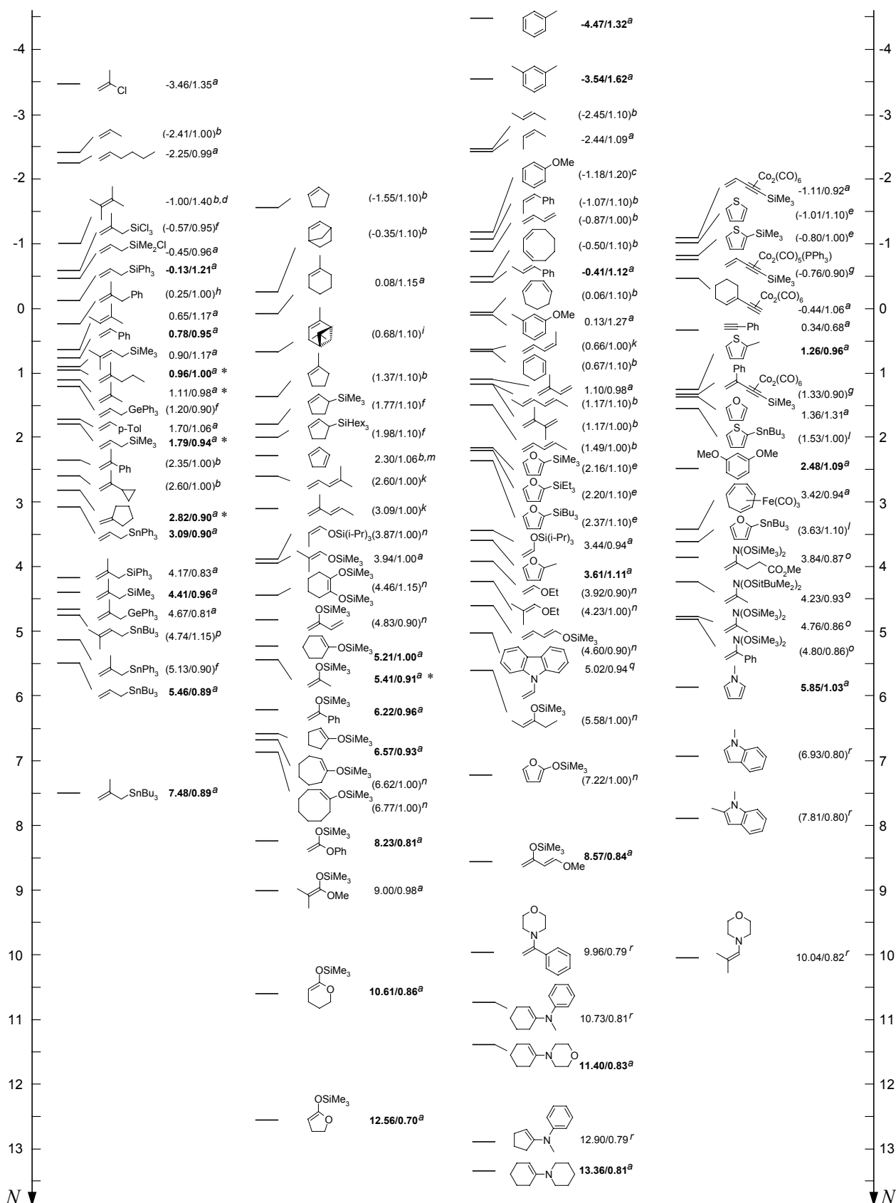
Figure 5. Nucleophilicity and slope parameters N/s for \pi -nucleophiles (04/2004). Reference compounds bold, parentheses indicate estimated values of s . For nucleophiles marked with an asterisk, additional reactivity parameters of structurally analogous compounds are listed in Table 1 of ref. #191. a From ref. #180. b-r For details of the kinetic measurements, see b ref. #96, c ref. #114, d ref. #97, e ref. #177, f ref. #105, g ref. #174, h ref. #102, i ref. [M. Roth, Dissertation, TH Darmstadt 1996], k ref. #144, l ref. #178, m ref. [T. Siegmund, Dissertation, LMU München 1999], n ref. #159, o ref. #176, p ref. [M. Hartnagel, Dissertation, TH Darmstadt 1997], q ref. #187, and r ref. #195.
