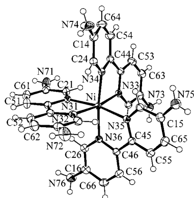
Figure 3. Exemplified view of the molecular structure of the tris(chelate)metal cations in [\text{Fe}(\mathbf{5})_3]\text{SO}_4 \times 9 \text{H}_2\text{O} ( 16 ), [\text{Ni}(\mathbf{5})_3]\text{Cl}_2 \times 2.5 \text{H}_2\text{O} ( 17 ), [\text{Ni}(\mathbf{5})_3](\text{SCN})_2 ( 18 , shown here), and in [\text{Zn}(\mathbf{5})_3](\text{NO}_3)_2 ( 22 ); selected distances and angles are given in Table 3
