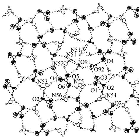
Figure 6. Two-dimensional hydrogen bonding network in [Zn(5) 3 ](NO 3 ) 2 ( 22 ) in the ab plane; the nitrogen atoms of the amino groups are drawn as empty ellipsoids only; due to space requirements only part of the atom positions are labelled and symmetry operations are not shown
