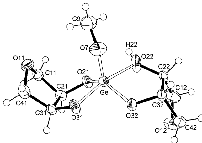
Figure 3 ORTEP diagram of \text{Ge}(\text{OCH}_3)(\text{AnErytH}_{-2})(\text{AnErytH}_{-1}) ( 3 ). Displacement ellipsoids are drawn at the 50% probability level. Crystal defects result in high electron density max data.
