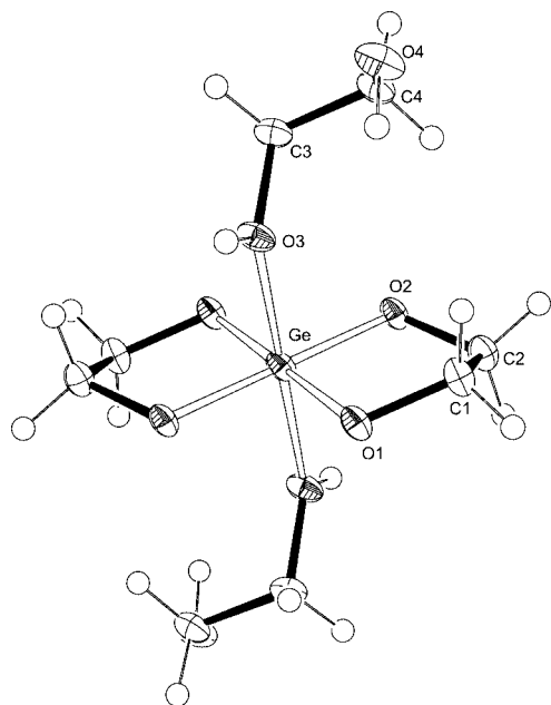
Figure 4 ORTEP diagram of \text{Ge}(\text{EthdH}_{-2})_2(\text{Ethd})_2 ( 4 ). Displacement ellipsoids are drawn at the 50% probability level.
