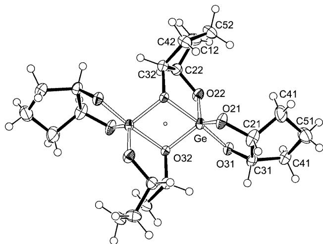
Figure 2 ORTEP diagram of the C_i symmetric molecule \{\text{Ge}(\text{cis-1,2-CptdH}_{-2})\}_2 ( 2 ). Displacement ellipsoids are drawn at the 50% probability level. The inversion center is indicated by a small circuit.
